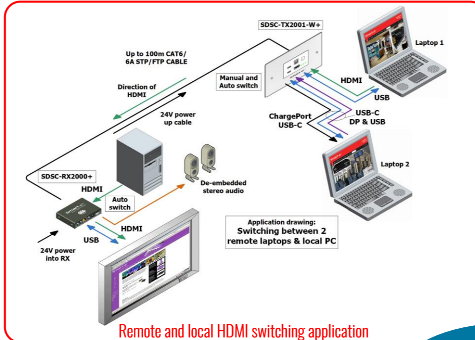
SDSC-2001+ Application drawing 1
