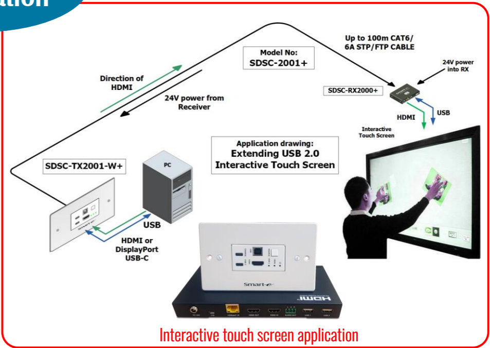
SDSC-2001+ Application drawing 2
