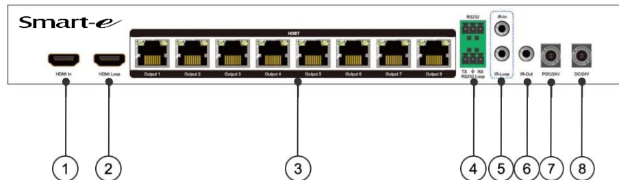
Rear Panel
